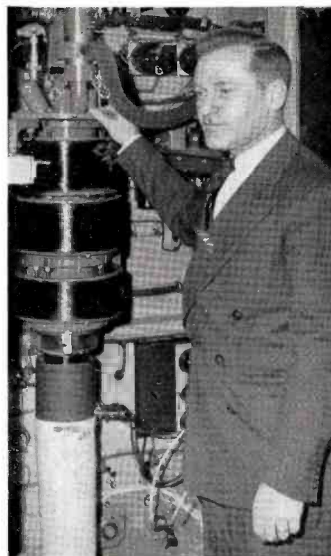
● Heart of Channel 61's powerful transmitter is the 15-kw G-E klystron tube at Chief Engineer Townsend's right. It airs WWLP's television signal over a wide radius. Clear pictures are further assured by the 320-foot transmitting tower based 640 feet high on Provin Mountain in the limits of the town of Agawam.
