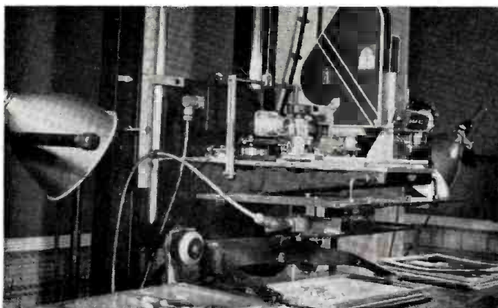
Fax automatic animation camera and crane.
